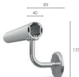
HR-6N-S75
