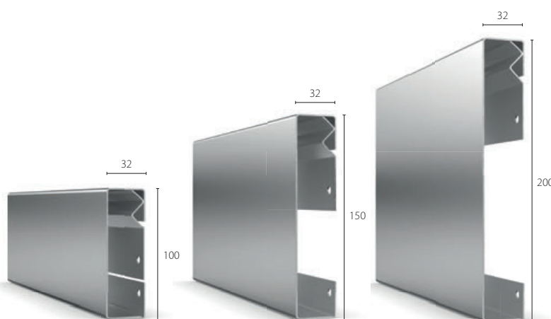
CRS-100
